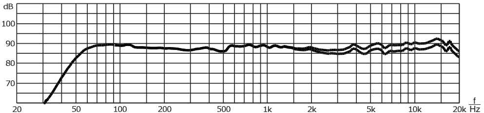
② Frequency response
