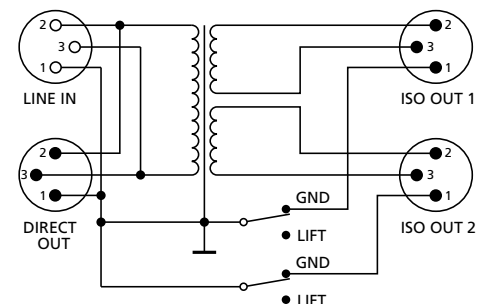
Principalschaltbild (1 Kanal) Basic circuit diagram (1 channel)
